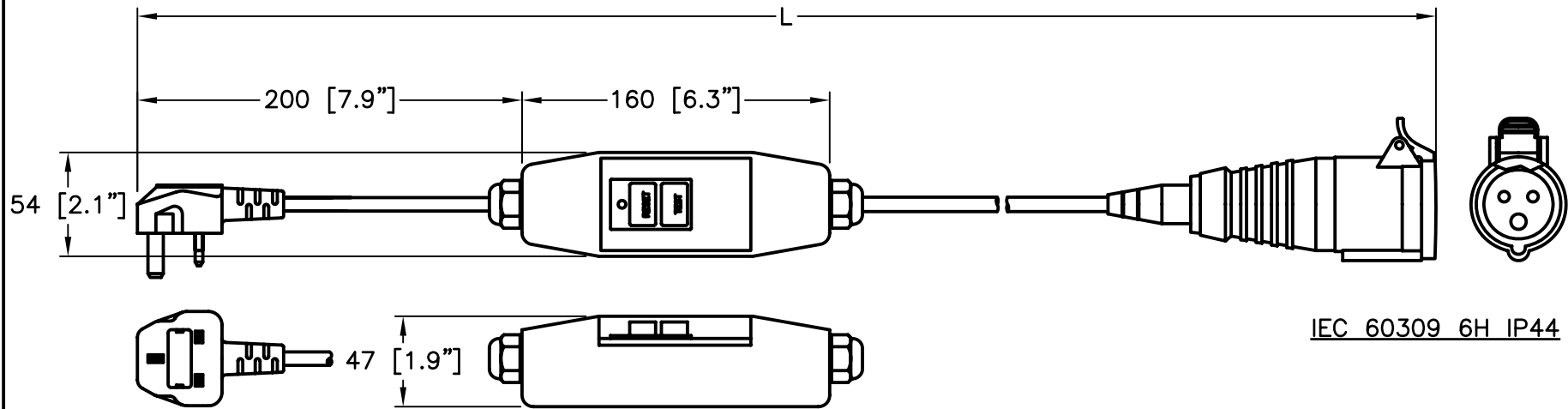
BS1363A
